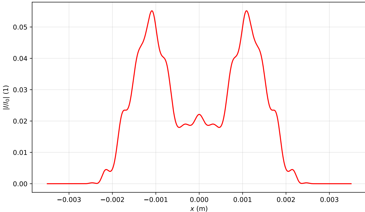
Intensity profile I(x, y = 0, z = 3.582)/I_0 , \text{Pin}=6.0\text{Pcr} , artificial time
